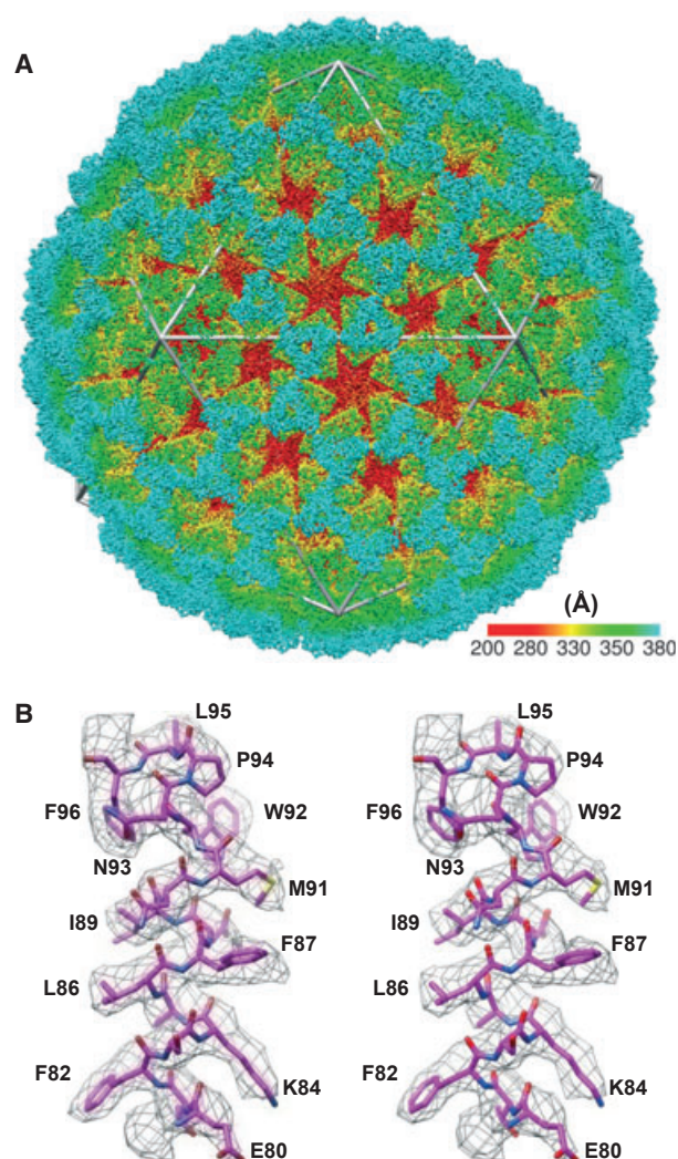
Fig. 7. Determination of the structure of a non-enveloped icosahedral virus using cryo-electron microscopy. Visualization of (A) the entire structure and (B) a selected region, demonstrating that near-atomic resolution maps may be obtained for highly ordered assemblies such as icosahedral viruses using advanced image-processing methods. Adapted from [19].
