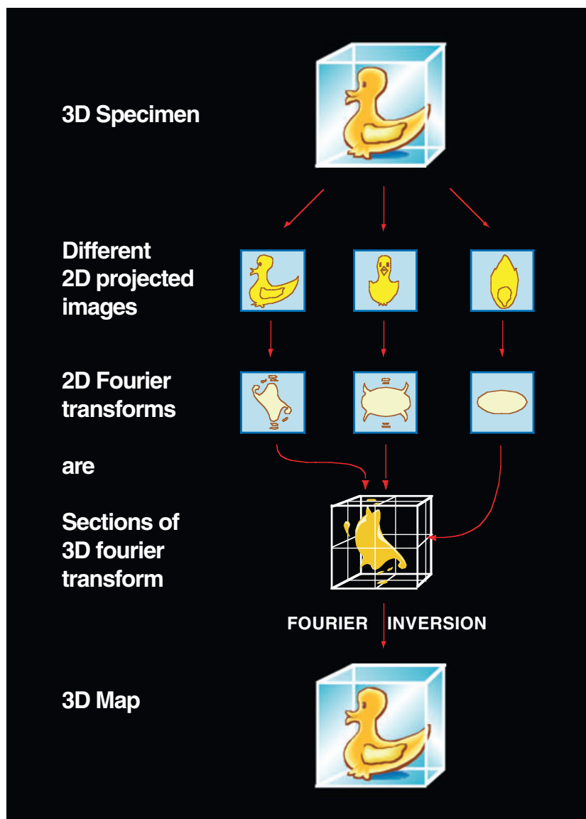
Fig. 5. Principle of reconstruction of 3D structure by Fourier inversion. Using the 'Fourier duck' as the prototypical biological specimen, the schematic shows that projection images of the object, each with a different orientation, have 2D Fourier transforms that correspond to sections (indicated by red arrows) through the 3D Fourier transform of the original object. Once the 3D Fourier transform is built up from a collection of 2D images spanning a complete range of orientations, Fourier inversion enables recovery of the 3D structure [91a].
