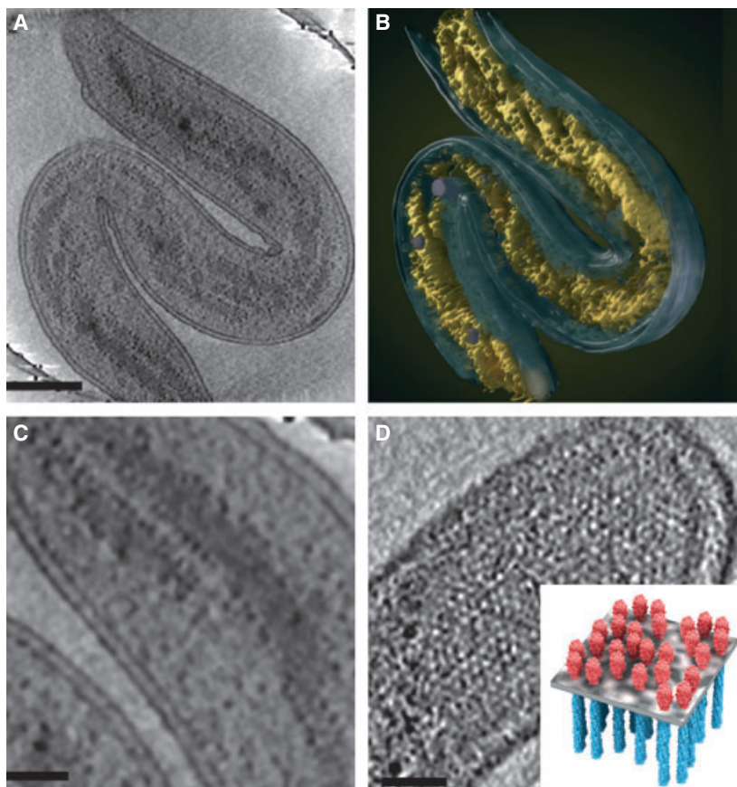
Fig. 2. Use of cryo-electron tomography to image the interior architecture of intact bacterial cells. (A, B) Illustration of the spiral architecture of the nucleoid in Bdellovibrio bacteriovorus showing (A) a 210 Å thick tomographic slice through the 3D volume of a cell, and (B) a 3D surface rendering of the same cell, with the spiral nucleoid highlighted (yellow). (C) Higher-magnification view of a tomographic slice through the cell, showing well-separated nucleoid spirals and ribosomes (dark dots) distributed at the edge of the nucleoid. (D) Expanded views of 210 Å thick tomographic slices, showing top views of polar chemoreceptor arrays. A schematic model (inset) illustrates the spatial arrangement of the chemoreceptor arrays in the plane of the membrane. Scale bars = 2000 Å (A) and 500 Å (C, D). Adapted from [44].
