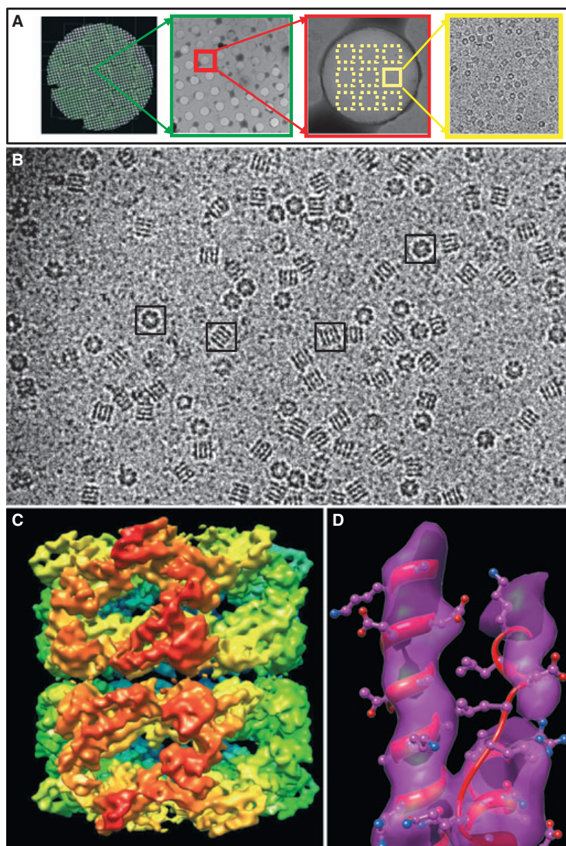
Fig. 6. Automation of macromolecular assembly structure determination by cryo-EM single-particle analysis. (A) Images of a cryo-EM grid at sequentially higher magnification, starting (left) with an image of the entire grid and concluding with an image of individual structures (right). (B) Representative projection image from a frozen-hydrated specimen of purified GroEL protein complexes. Complexes with distinct orientations relative to the electron beam may be discerned, as indicated in the boxed examples. (C) 3D reconstruction using approximately 28 000 individual projection images such as those boxed in (B) to generate a density map of the complex at approximately 7 Å resolution. The initial 3D reconstruction was derived by sub-volume averaging using approximately 2000 GroEL particles. Refinement of the initial reconstruction was performed using almost completely automated procedures as implemented in the software package FREALIGN [87a] to refine the structure to approximately 7 Å resolution. (D) Demonstration that the resolution achieved is adequate to visualize \alpha -helices, illustrated by superposition of a density map of a region of the polypeptide on the corresponding region of a GroEL structure determined by X-ray crystallography (PDB ID: 3E76 ). Panels (B–D) provided by A. Bartesaghi, unpublished results.
