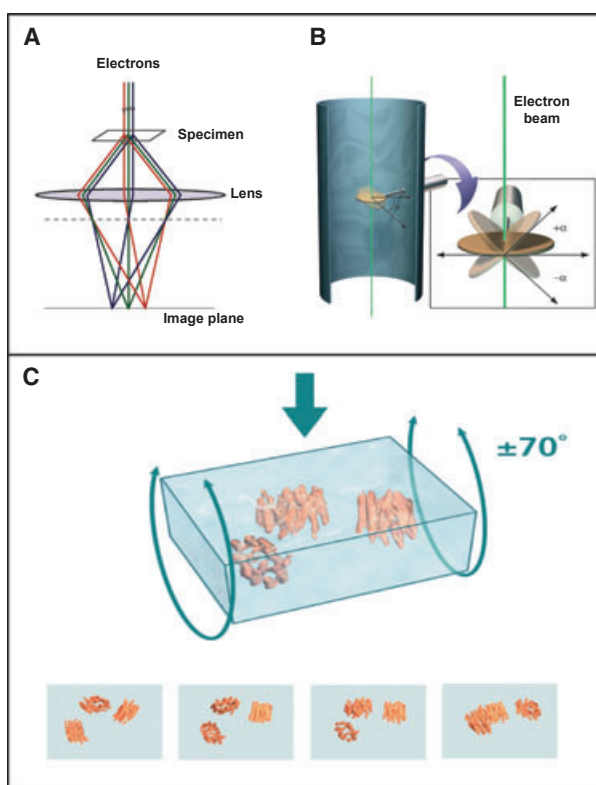
Fig. 1. Image formation in the electron microscope. (A) Schematic illustrating image formation in an electron microscope, highlighting the similarities between electron and optical microscopy. (B) Schematic illustrating the principle of data collection for electron tomography. As the specimen is tilted relative to the electron beam, a series of images is taken of the same field of view. (C) Selected projection views generated during cryo-electron tomography as a vitrified film (formed by rapidly freezing a thin aqueous suspension) is tilted relative to the electron beam. To reconstruct the 3D volume, a set of projection images is ‘smeared’ out along the viewing directions to form back-projection profiles. The images are combined computationally to obtain the density distribution of the object. Adapted from [110].
