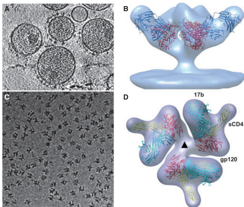
Fig. 4. Structural analysis of membrane protein complexes using cryo-electron tomography combined with sub-volume averaging. (A) Tomographic slice through a field of HIV virions recorded from a specimen grid that was plunge-frozen and stored at liquid nitrogen temperatures. In this image, the viral membrane is decorated with trimeric envelope glycoproteins, which are required for viral entry into target cells. (B) Density map at approximately 20 Å resolution of the trimeric envelope glycoproteins complexed with the neutralizing antibody VRC01. The map was obtained by missing-wedge corrected, sub-volume averaging of cryo-electron tomographic images. The map was then fitted with three copies of the X-ray crystallographically determined structure for the complex of monomeric gp120, a portion of the HIV envelope glycoprotein, complexed with VRC01. (C) Projection image of individual molecular complexes of soluble trimeric envelope glycoproteins from HIV strain KNH1144. (D) Density map at approximately 20 Å resolution of the complex of HIV envelope glycoproteins (molecular weight of polypeptide portion approximately 240 kDa) with soluble CD4 (molecular weight approximately 24 kDa) and Fab fragment (molecular weight approximately 50 kDa). The map is fitted with three copies of the structure of the ternary complex of monomeric gp120, sCD4 and 17b Fab determined by X-ray crystallography. Adapted from [73] and [74].
