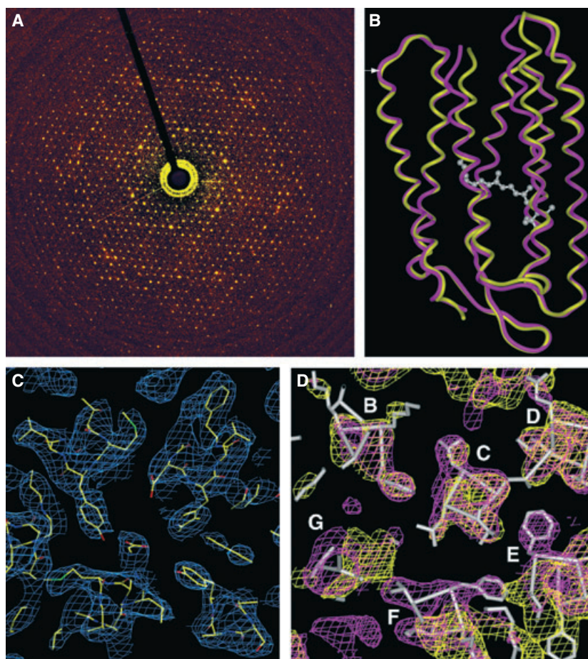
Fig. 8. Determination of membrane protein structure using electron crystallography of 2D crystals. (A) Electron diffraction pattern from bacteriorhodopsin crystals, with reflections extending to approximately 2 Å. (B) Structures of bacteriorhodopsin in native and intermediate conformations at 3.2 Å resolution were obtained by combining phase information present in images of 2D crystals with amplitude information obtained from electron diffraction patterns. (C) \sigma_A -weighted density ( 2F_O - F_C ) map of the open intermediate of bacteriorhodopsin in the center of a lipid bilayer. The map is fitted with the refined atomic model (PDB ID: 1FBK ). (D) Sections of bacteriorhodopsin in wild-type (purple) and open intermediate (yellow) conformations, showing the helix movements (from magenta to yellow coordinates) at the cytoplasmic ends of transmembrane helices F and G. The location of the section is indicated by the white arrow at the left edge of (B). The maps are superimposed on the structure of wild-type bacteriorhodopsin, derived by cryo-electron microscopy at 3.2 Å resolution. Figure adapted from [16].
