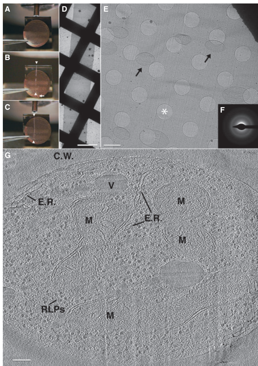
Fig. 3. Imaging of vitreous sections by cryo-electron microscopy. (A) An EM grid is placed at the diamond knife edge using tweezers with a bent tip. (B) A ribbon of vitreous sections (white arrowheads) is guided over the EM grid using an eyelash (white arrow) attached to a wooden dowel. (C) Once the ribbon of vitreous sections is of suitable length (white arrowheads) (approximately the diameter of the EM grid), an electrostatic generator is switched from discharge mode to charge mode, causing the ribbon to attach to the EM grid. (D) Low-magnification image showing the ribbon of vitreous sections after electrostatic charging. Scale bar = 50 \mu\text{m} . (E) Medium-magnification micrograph showing a vitreous section from within the ribbon. Note that the section is smooth and relatively flat, with no apparent mechanically induced damage as is often seen with stamping/pressing techniques. S. cerevisiae cells may be seen scattered throughout the vitreous section (black arrows). Holes within the C-Flat EM grid (Protochips Inc., Raleigh, NC) may be seen, one of which is indicated by a white asterisk. Scale bar = 2 \mu\text{m} . (F) A selected area diffraction pattern indicating the presence of vitreous ice. (G) A 50 \text{\AA} thick slice through a reconstructed tilt series from a 500 \text{\AA} thick vitreous section of an S. cerevisiae cell: C.W., cell wall; V, vacuole; M, mitochondrion; E.R., pieces of endoplasmic reticulum; RLPs, ribosome-like particles. Scale bar = 1000 \text{\AA} . Adapted from [49].
