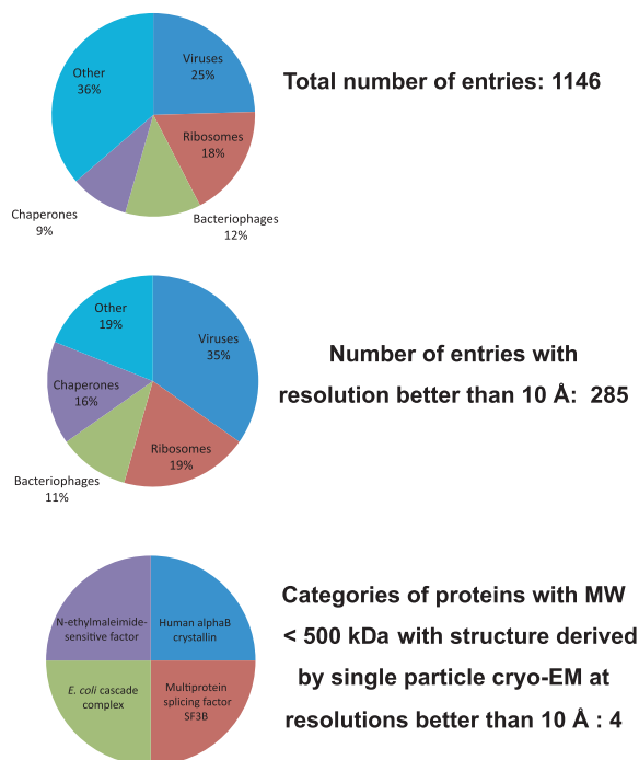
Fig. 9. Distribution of released entries belonging to the ‘single-particle’ and ‘icosahedral’ categories in the EMDB ( http://emdatbank.org/ ) as of June 2012. Structures from ribosomes and icosahedral viruses dominate the deposited entries, both in the entire dataset, and even more strikingly, in the subset of entries with resolutions better than 10 Å. Further inspection shows that there are only four distinct protein complexes with molecular masses < 500 kDa (multiprotein splicing factor SF3B, EMD-1043; DegQ, EMD-5290; Escherichia coli cascade complex, EMD-5314 and EMD-5315; N -ethylmaleimide-sensitive factor, EMD-5370 and EMD-5371), thus identifying a key gap in structural biology that may potentially be filled by taking advantage of improvements in microscope hardware and algorithms for image processing.
